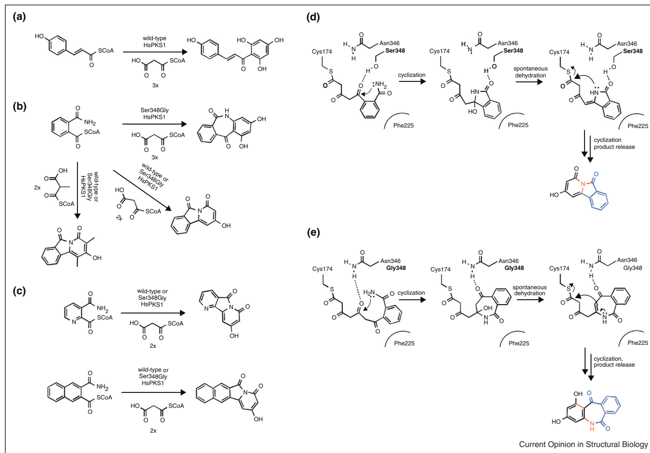
Wild-type and engineered type II PKS HsPKS1 for the synthesis of unnatural alkaloids. (a) Native reaction catalyzed by the wild-type HsPKS1. (b) Substrate and catalytic versatility of the wild-type and mutant HsPKS1. (c) Starter unit promiscuity of HsPKS1. (d) Proposed catalytic mechanism for formation of the 6.5.6-fused tricyclic ring system by wild-type HsPKS1. (e) Proposed catalytic mechanism for formation of the 6.7.6-fused ring system by the engineered HsPKS1.
