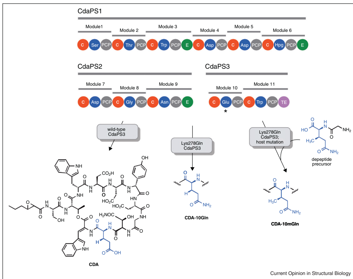
Organization of the NRPS responsible for CDA biosynthesis. Shown are the products of the wild-type and engineered NRPS. The module targeted for mutagenesis is highlighted with an asterisk.
